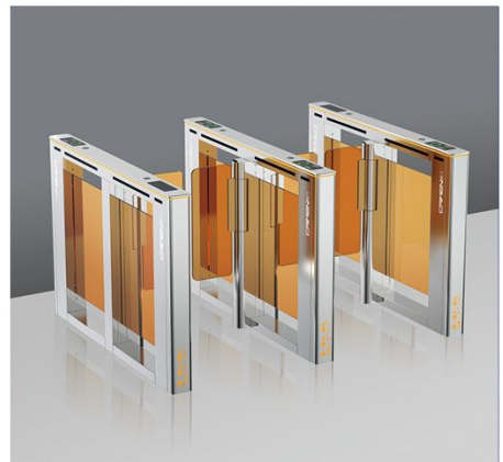
ST001 Speed Gate Turnstile Length:1400mm Width:120mm Height:980mm
